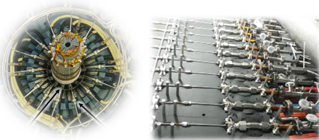
Figure 22: Higher radiation levels and new coolants will require identification and validation of suitable hardware and instrumentation solutions for the cooling circuits.
