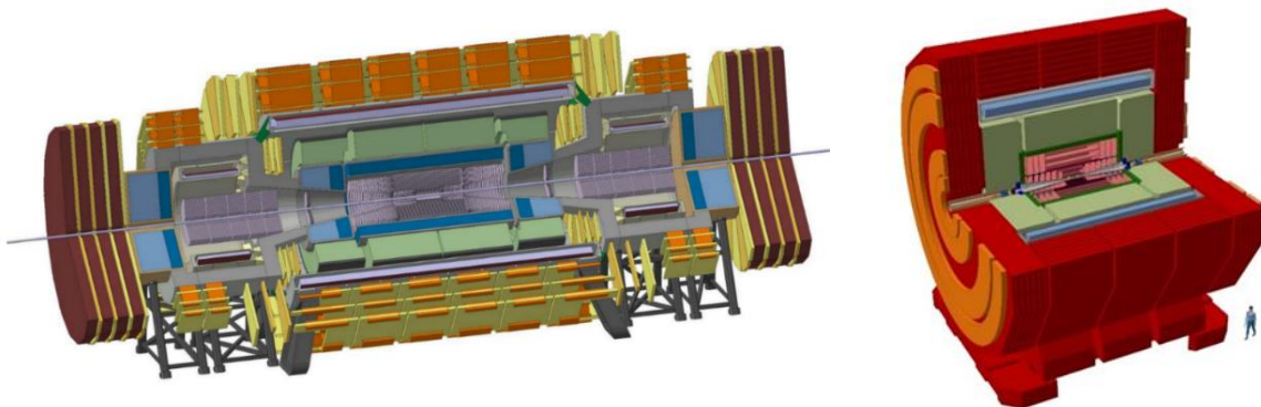
Figure 32 : Two detectors: the FCC-hh (left) and the CLICdp (right).
